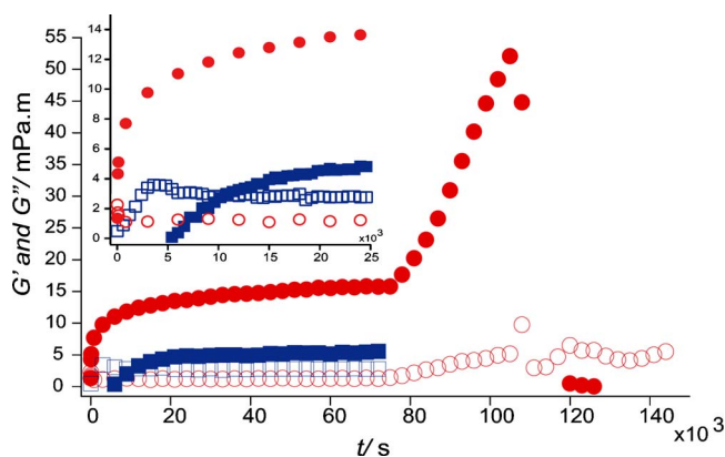
FIG. 3. (Color online) Time dependence of G' and G'' for spider silk (●) at 6% of strain and \beta -lactoglobulin (■) at 1.2% of strain. Full symbols represent G' and empty symbols G'' . The spider-silk concentration is at 0.02 \text{ mg/ml} . The \beta -lactoglobulin concentration is at 0.1 \text{ mg/ml} . At 72 000 s, phosphate ( 300 \text{ mM} ) was added in the aqueous phase of the spider-silk film to induce \beta -sheet formation. The inset is a zoom of the adsorption process at short times.
