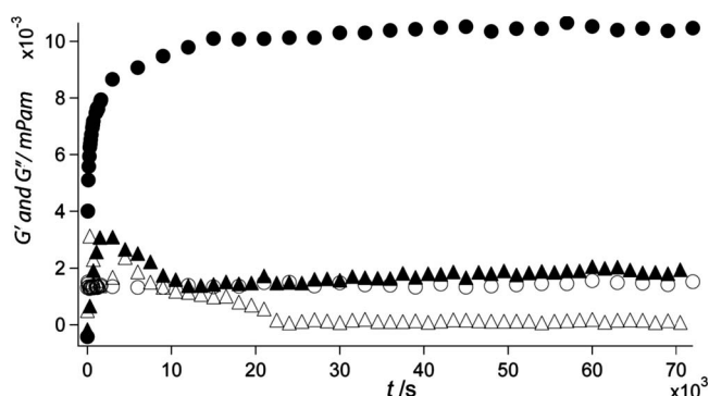
FIG. 5. Time dependence of G' and G'' during the competitive adsorption of spider silk and either dextran or lecithin. Black symbols represent G' and empty symbols represent G'' . \bullet : spider silk at 0.02 mg/ml and dextran at 20 mg/ml. \blacktriangle : spider silk at 0.02 mg/ml and lecithin at 10 \mu M.
